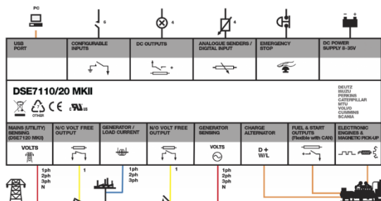
CONNECTION DIAGRAM
